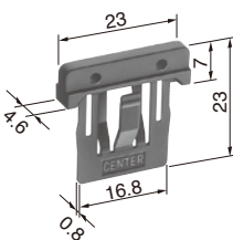
Center Barrier for Guard Cover
